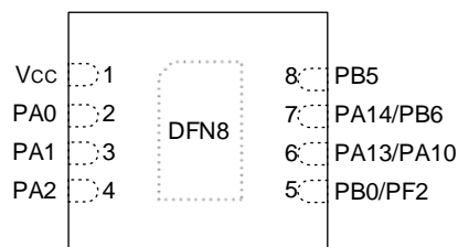
Figure 3-16 DFN8(1.5*1.5) Pinout1 PY32F030L1xDx / PY32F030L1xDx-E (Top view)
