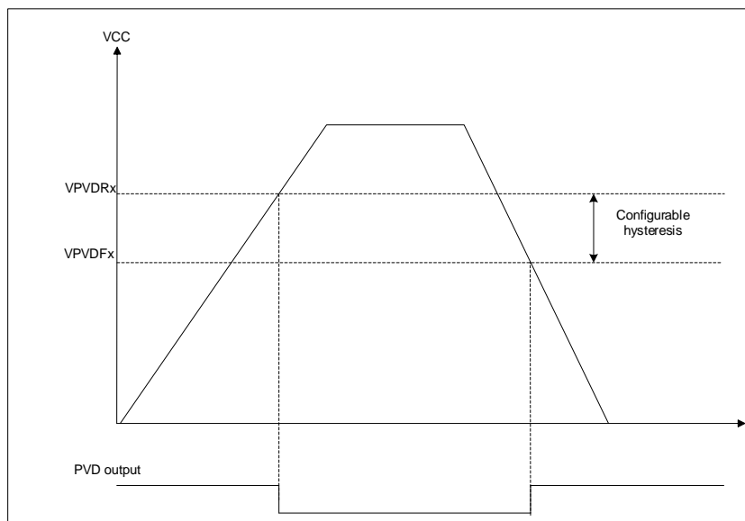
Figure 2-4 PVD Threshold
